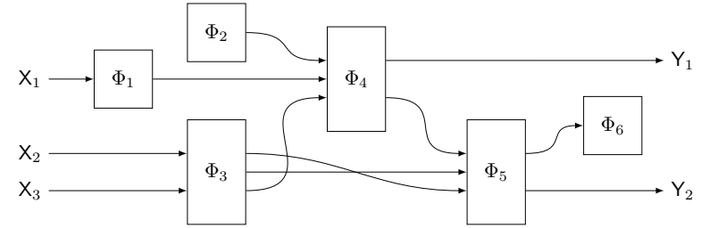
Figure 3.1 A hypothetical example of an acyclic network of channels. The arrows represent registers, and one assumes the input and output spaces of the channels (represented by rectangles) are compatible with the registers represented by the arrows. For instance, the channel \Phi_1 transforms the register X_1 into some other register (not explicitly named in the figure), which is the second of three inputs to the channel \Phi_4 . By composing the channels \Phi_1, \dots, \Phi_6 in the manner suggested by the figure, one obtains a single channel \Phi \in C(\mathcal{X}_1 \otimes \mathcal{X}_2 \otimes \mathcal{X}_3, \mathcal{Y}_1 \otimes \mathcal{Y}_2) .
